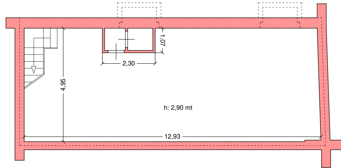
PIANO INTERRATO
